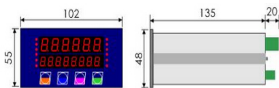
Front Panel
